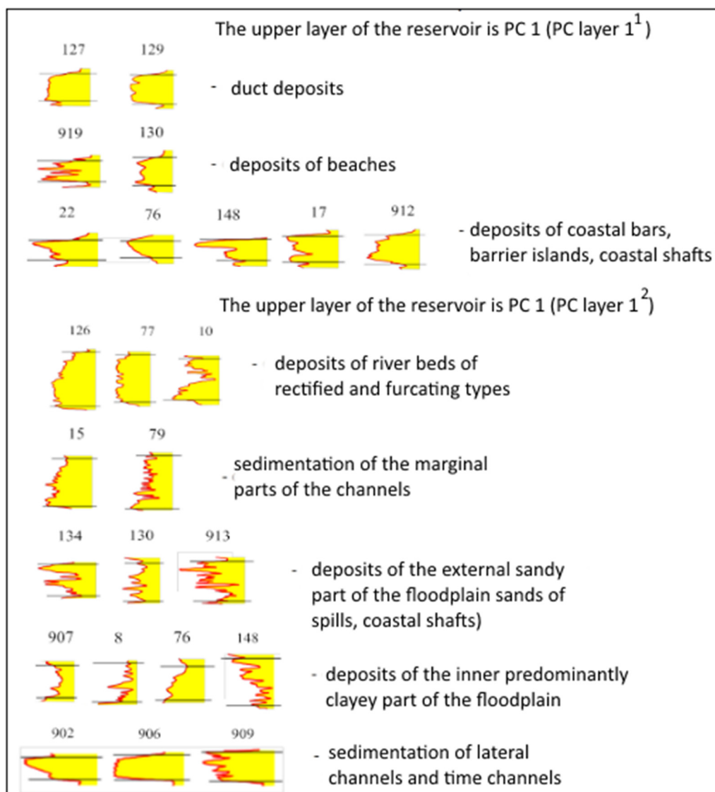
Figure 3. Electrometric models of facies of formation PC 1
