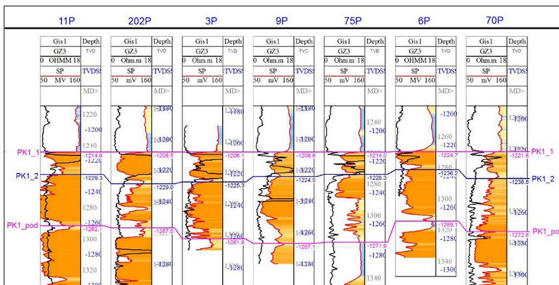
Figure 1. Scheme of correlation in the interval of formation PC_1
