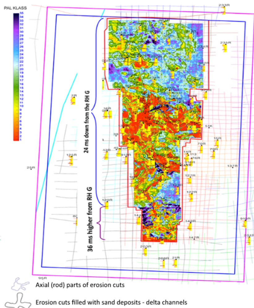
Figure 9. Horizontal sections by volume classification in the interval of the lower layer of the reservoir PC_1 ( PC\ layer_1^2 )
