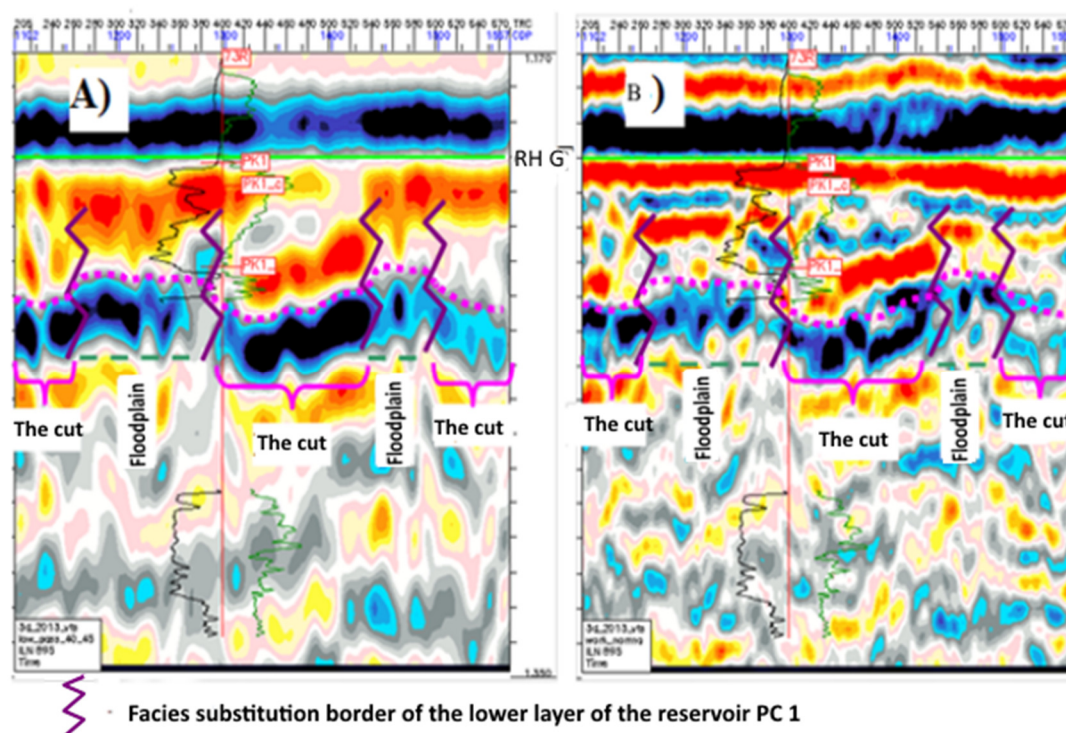
Figure 7. Fragment of the time section: A – filtered cube with BCA; B – high-frequency cube with BCA
